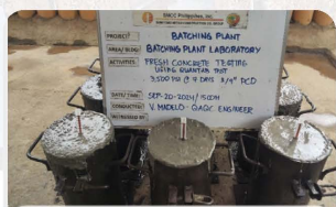
Quantab test for Freshly Batched Concrete Design for 3500 psi
