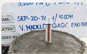
Setting of 3 Quantabs (3 Trials) one on each container with concrete set for 10 minutes
